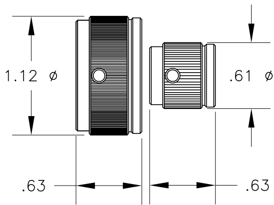
KNOB DETAIL
