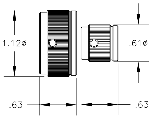
KNOB DETAIL
