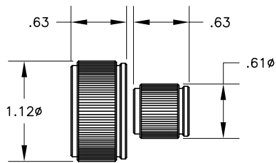
KNOB DETAIL
