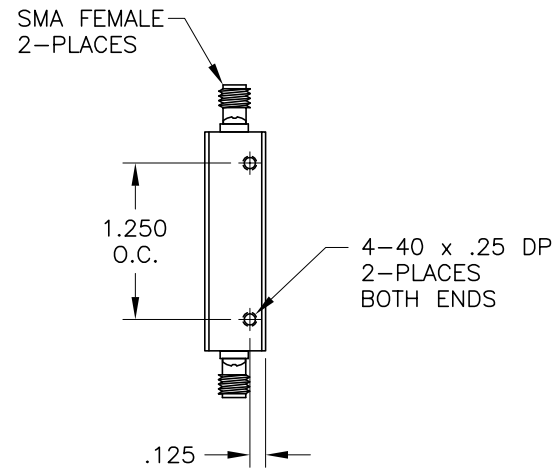
DETAIL A T&B #609-1057
