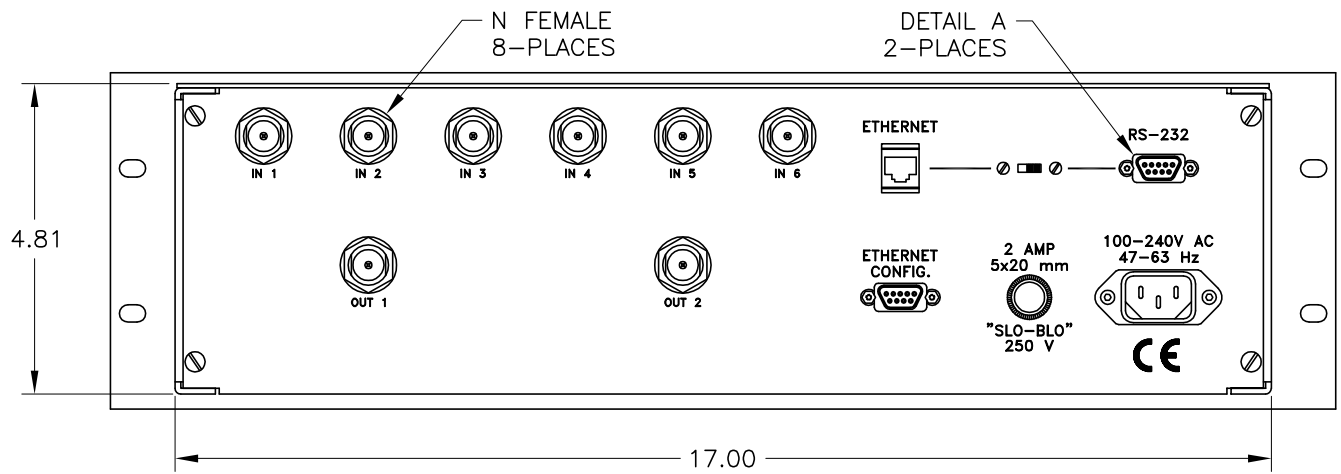
REAR VIEW
