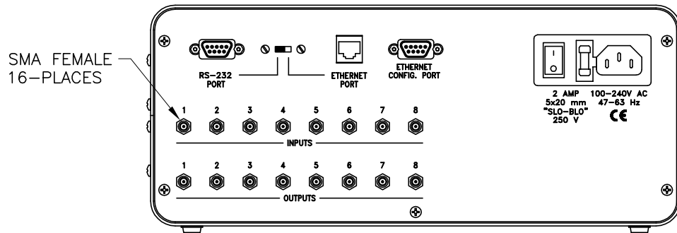
REAR VIEW
