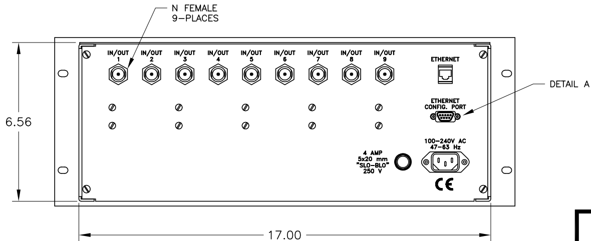
REAR VIEW
