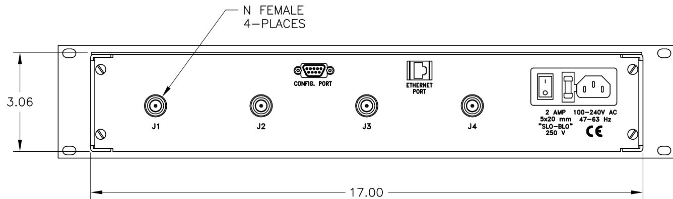
REAR VIEW
