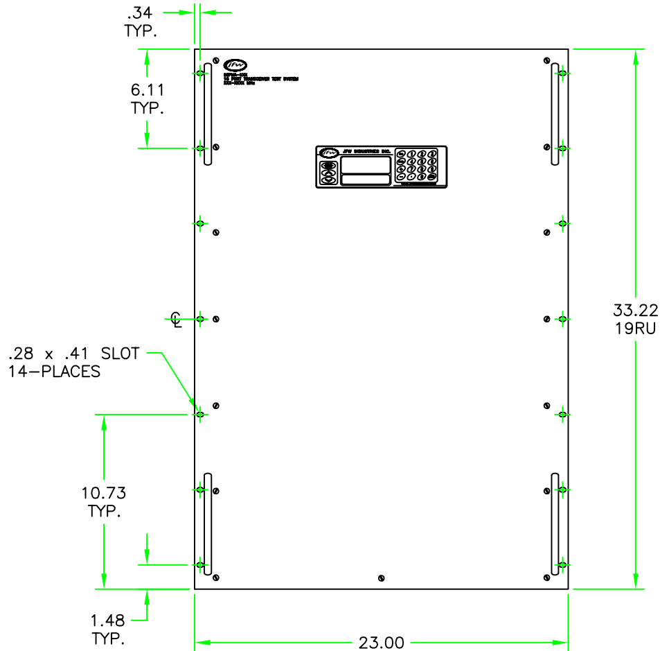
FRONT VIEW
