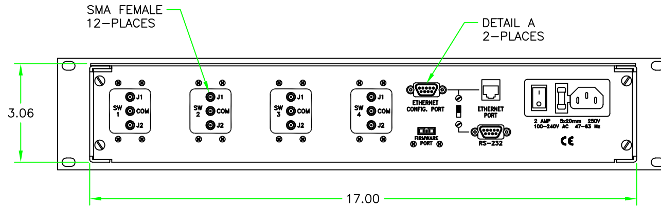
REAR VIEW
