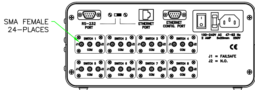
REAR VIEW
