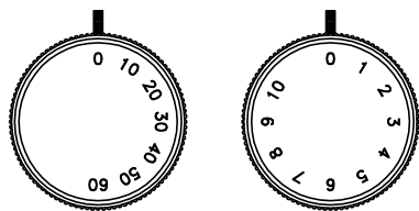
KNOB DETAIL
