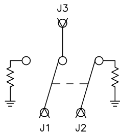
SHOWN WITH NO POWER APPLIED
