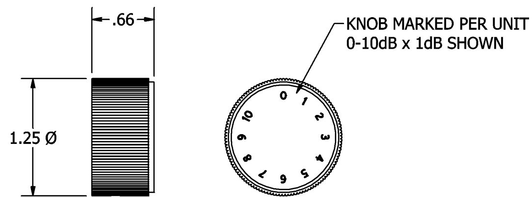
KNOB DETAIL
