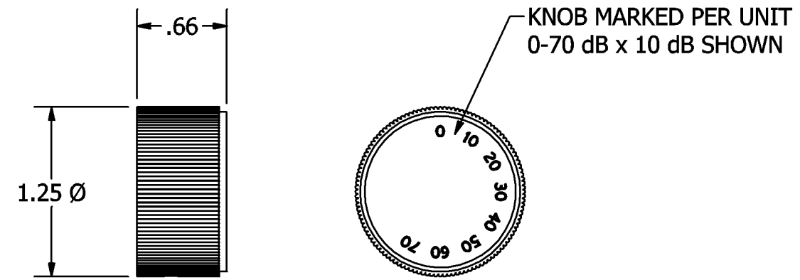
KNOB DETAIL
