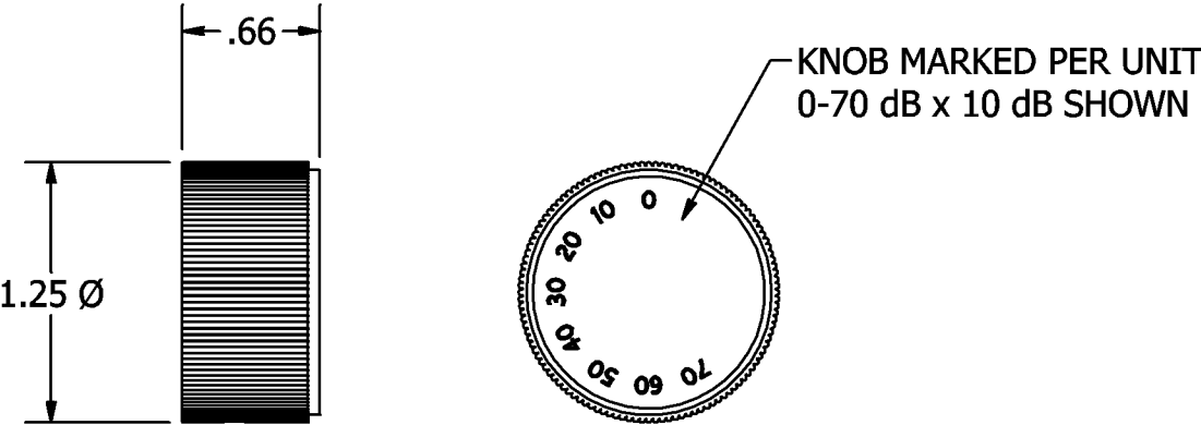
KNOB DETAIL
