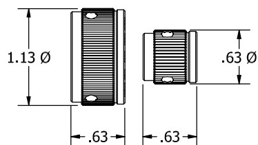
KNOB DETAIL
