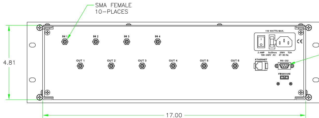
REAR VIEW
