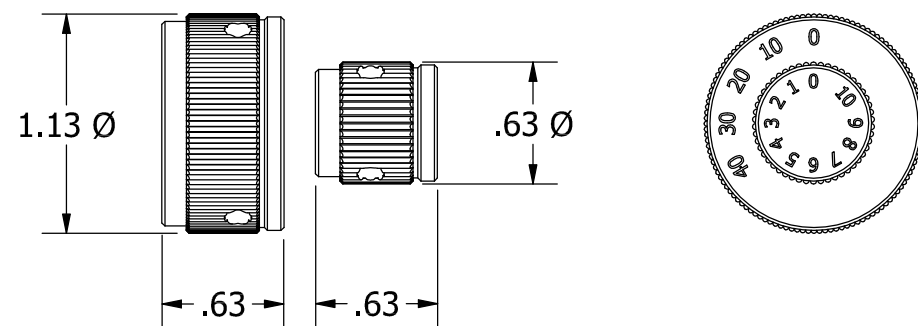
KNOB DETAIL
