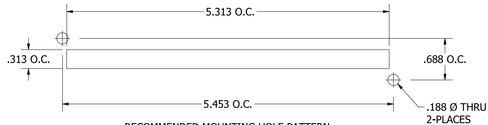
RECOMMENDED MOUNTING HOLE PATTERN
