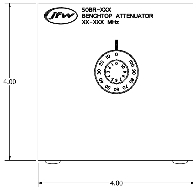
FRONT PLATE
