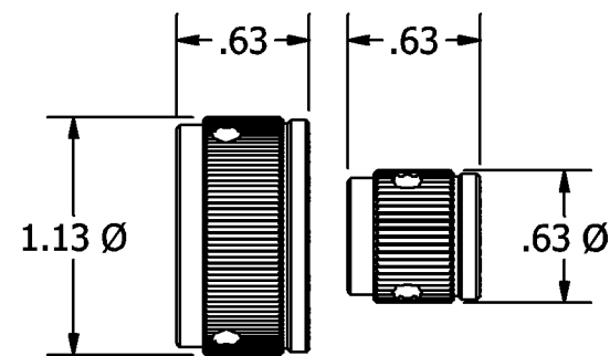
KNOB DETAIL
