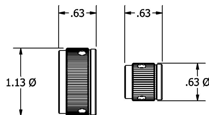
KNOB DETAIL
