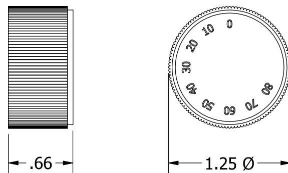
KNOB DETAIL
