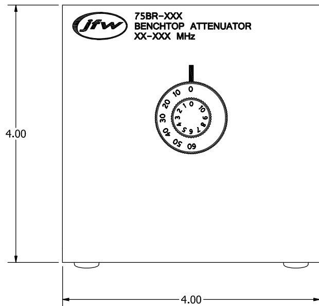
FRONT PLATE
