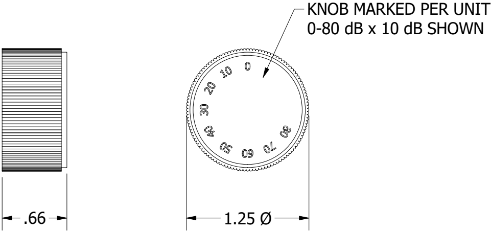
Knob Detail
