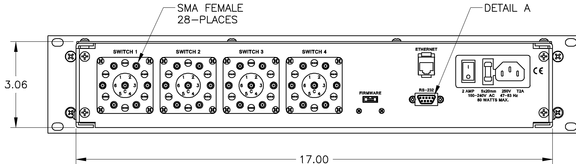
REAR VIEW
