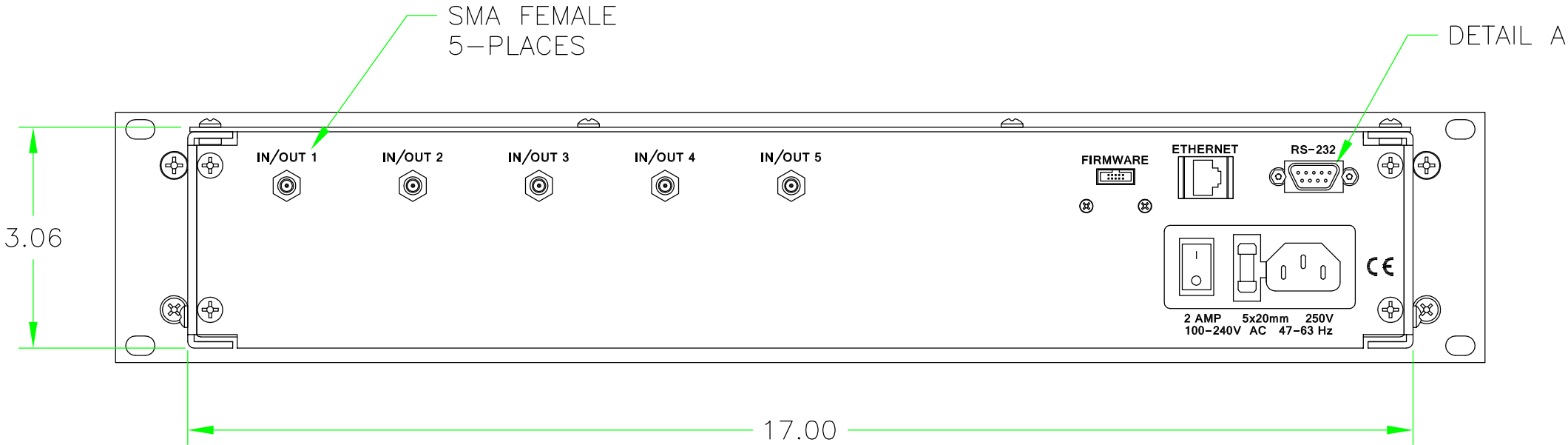
REAR VIEW
