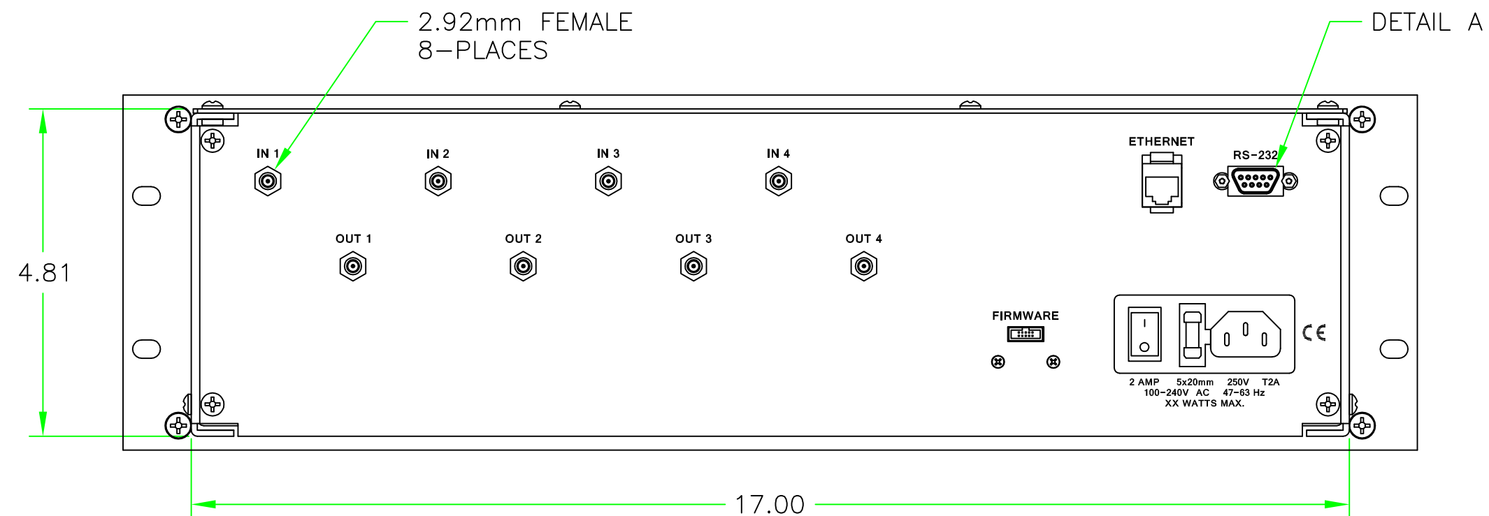
REAR VIEW
