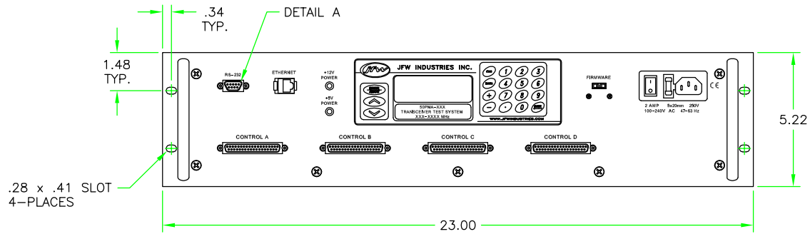
FRONT VIEW (CONTROL MODULE) CHASSIS DEPTH = 12.12
