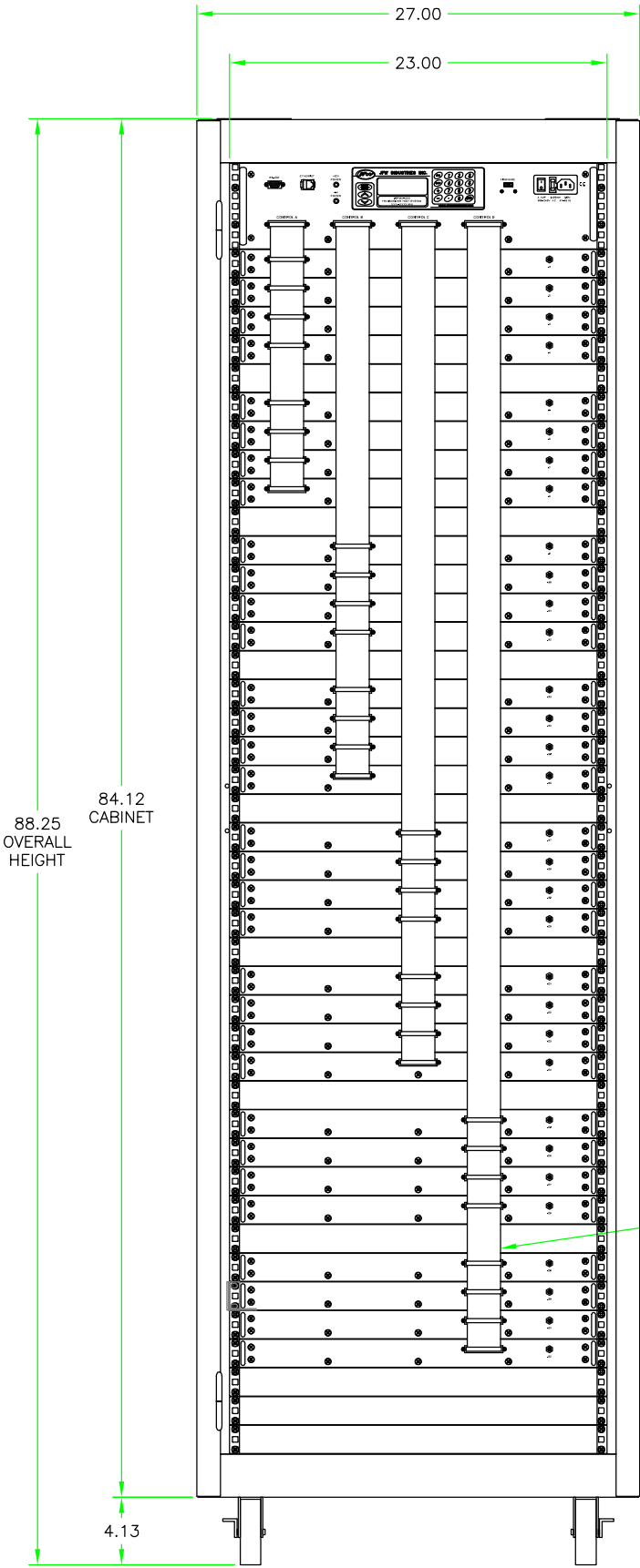
FRONT VIEW (DOOR NOT SHOWN)
