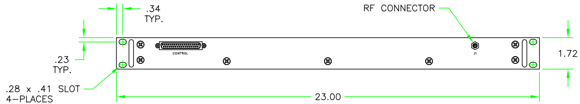
FRONT VIEW (MATRIX MODULE) CHASSIS DEPTH = 13.12
