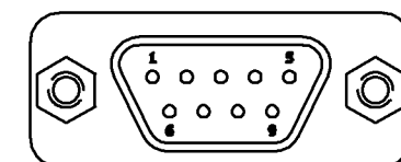
DETAIL A DE-9P
