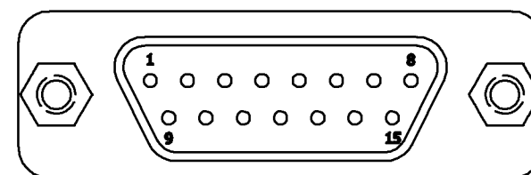
DETAIL A DA-15P
