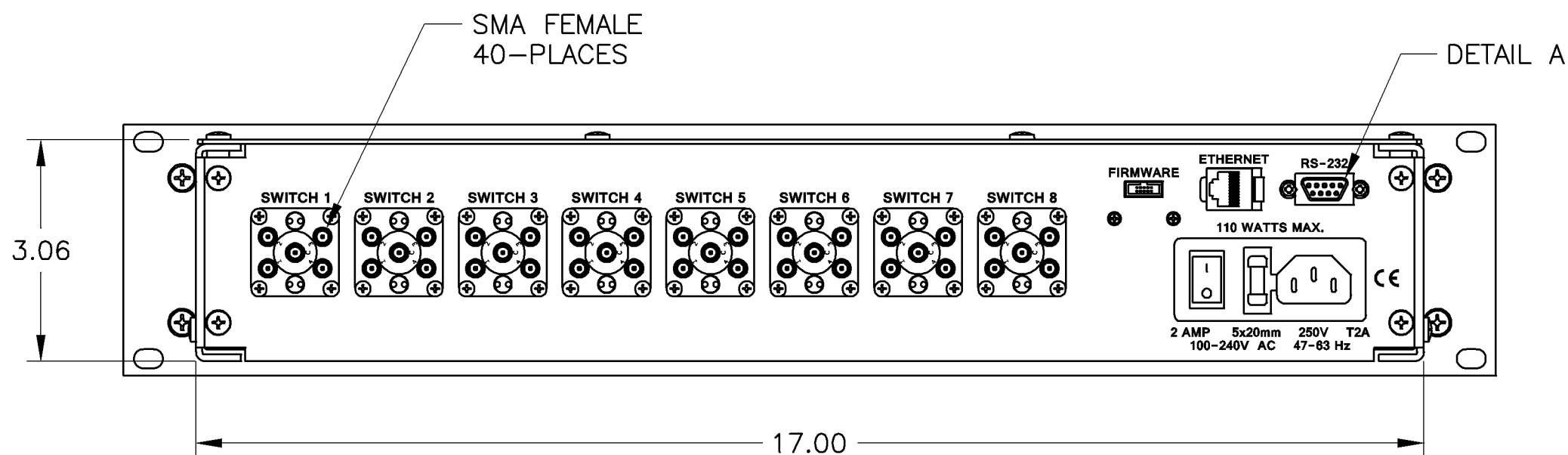
REAR VIEW
