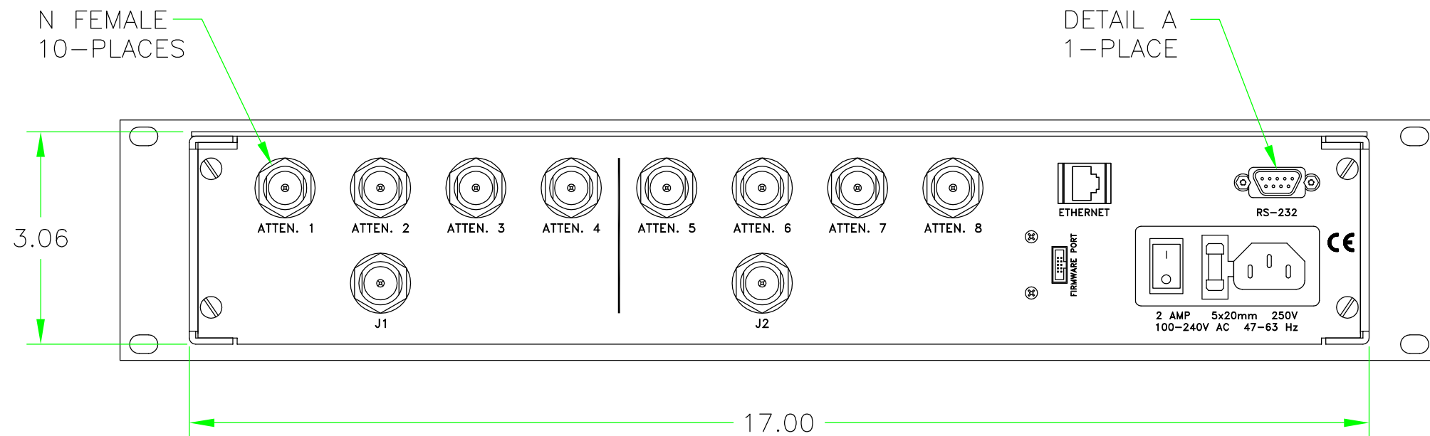
REAR VIEW
