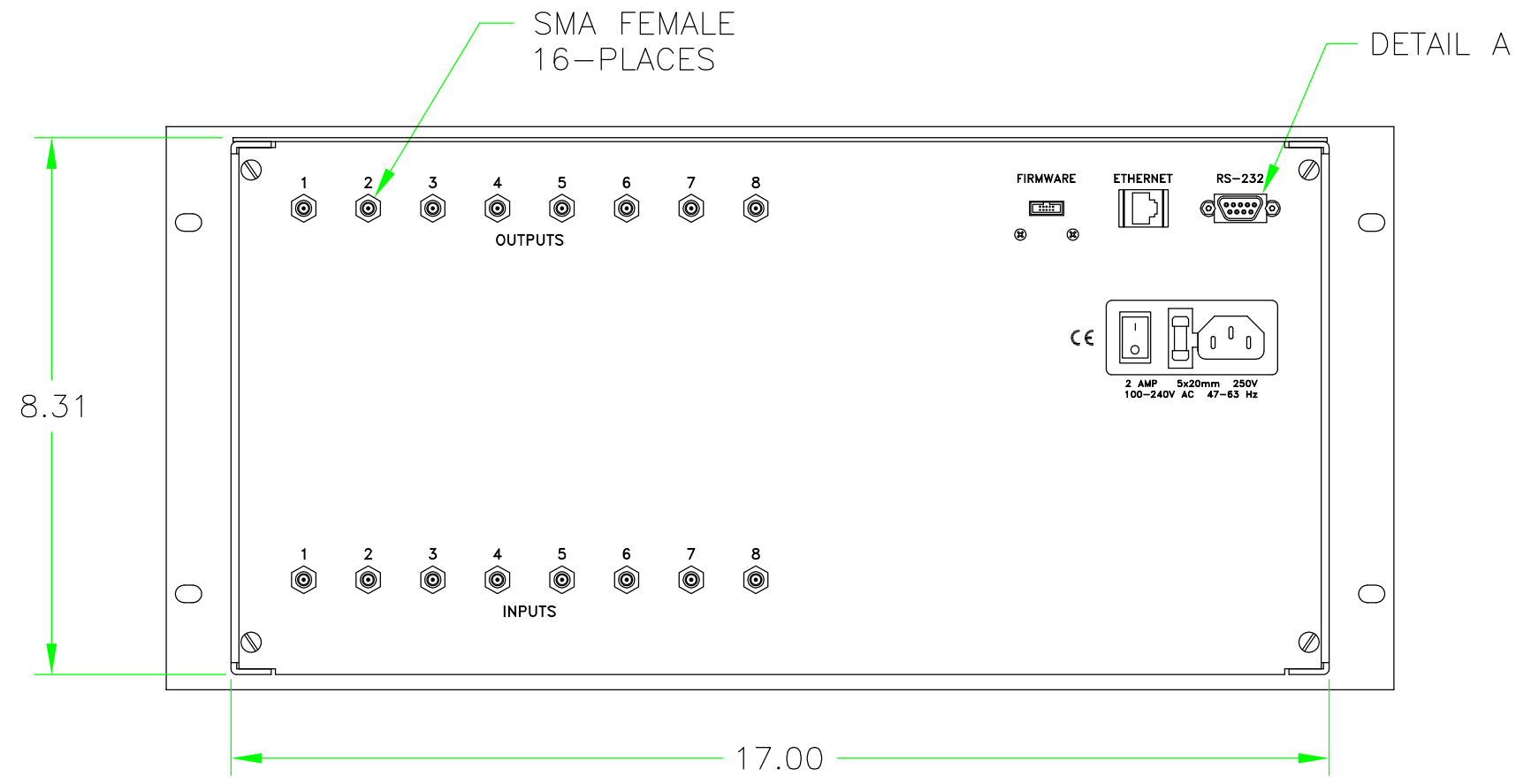
REAR VIEW
