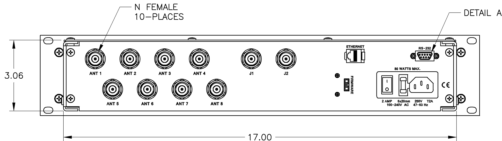
REAR VIEW
