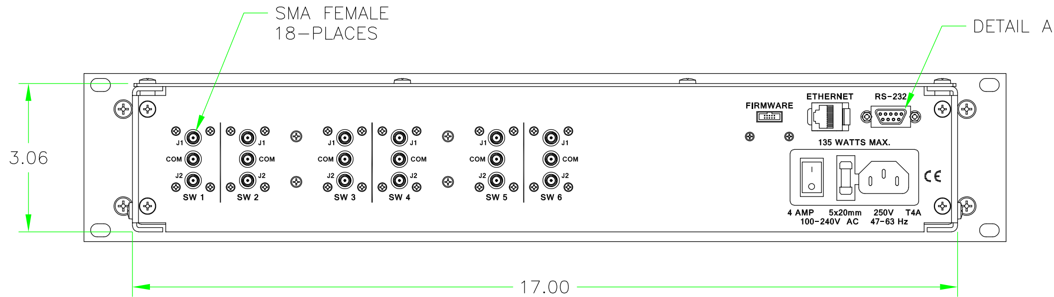
REAR VIEW
