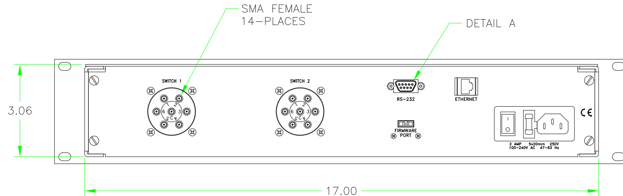
REAR VIEW
