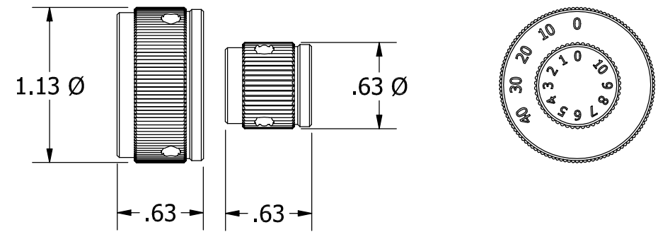
KNOB DETAIL
