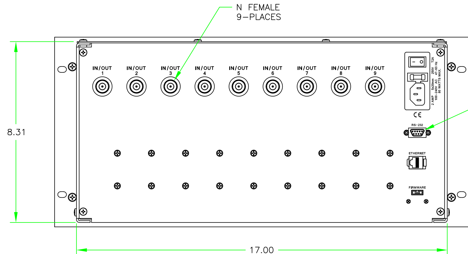
REAR VIEW
