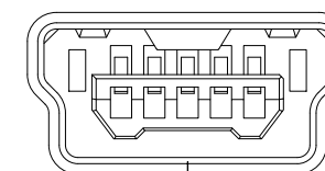
1 2 3 4 5 DETAIL A USB MINI-B
