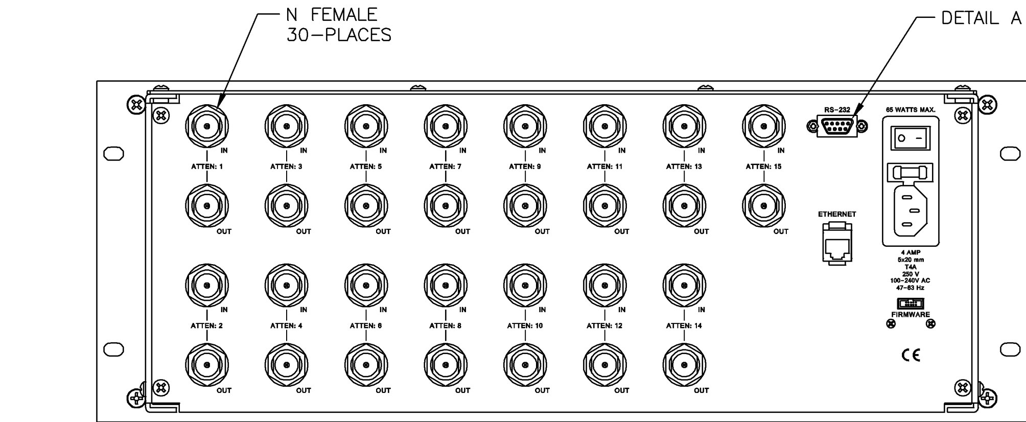
-15 (i.e. 15 ATTENUATORS)
