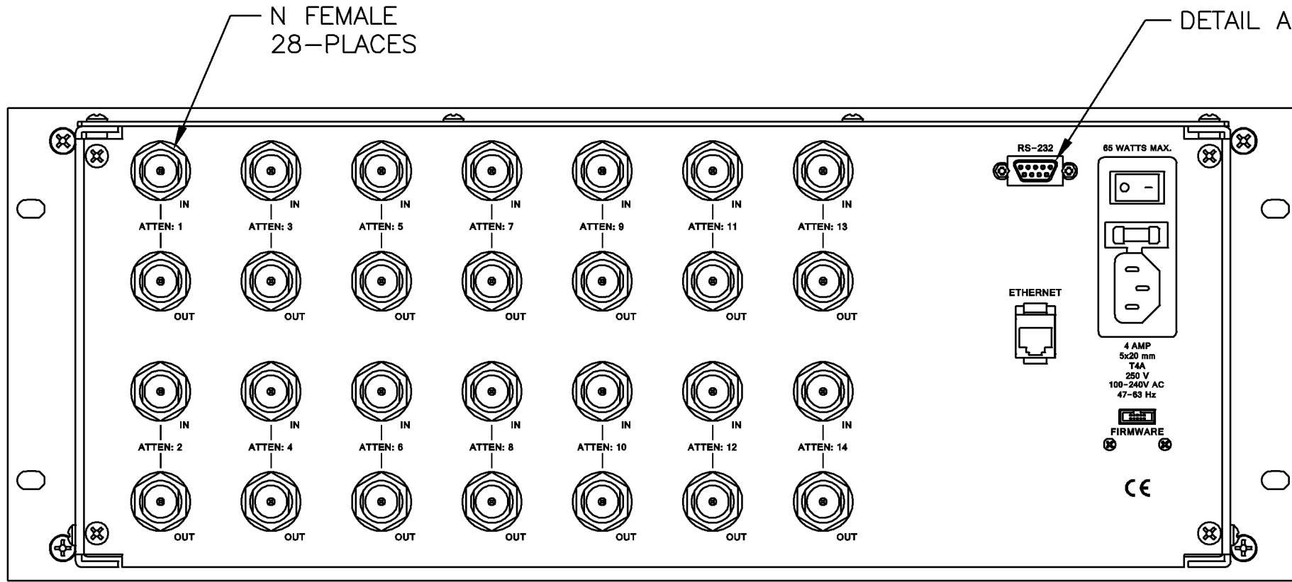
-14 (i.e. 14 ATTENUATORS)
