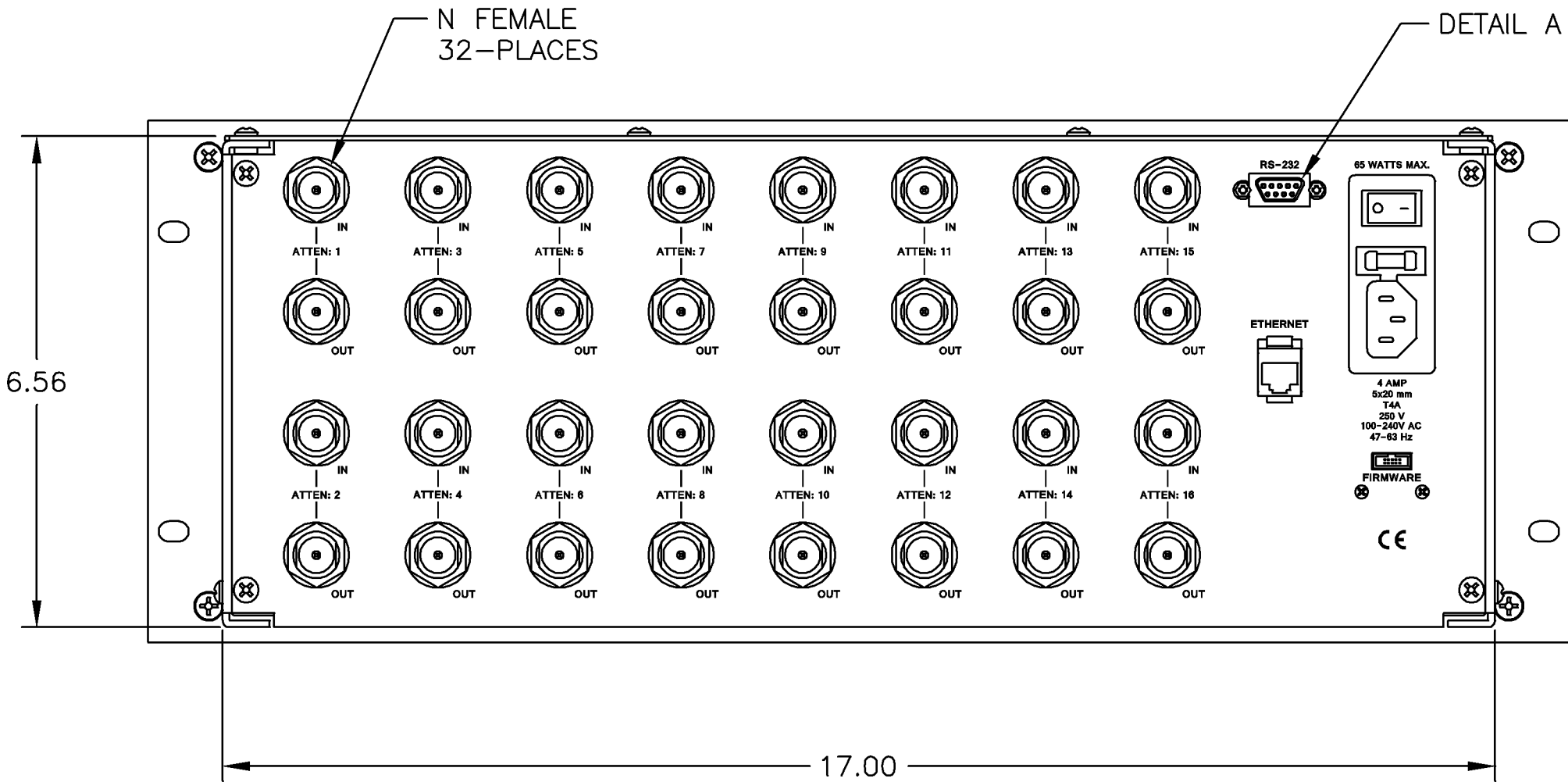
REAR VIEW
