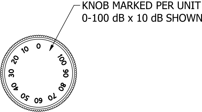
KNOB DETAIL
