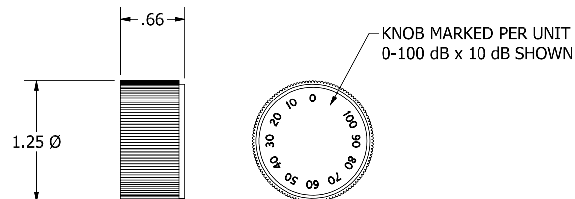
KNOB DETAIL
