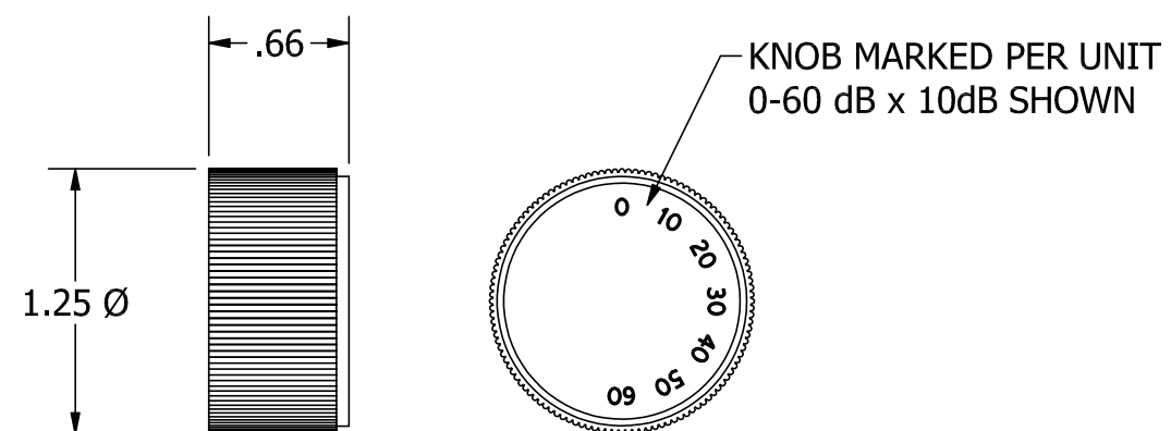
KNOB DETAIL
