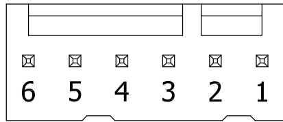
DETAIL A MOLEX #22-11-2062
