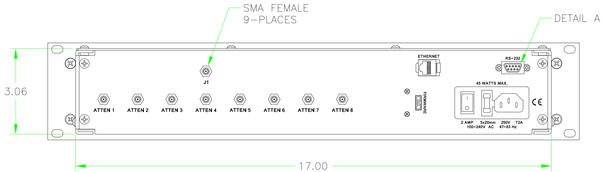
REAR VIEW
